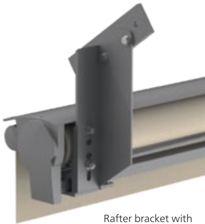
Rafter bracket with installation plate
