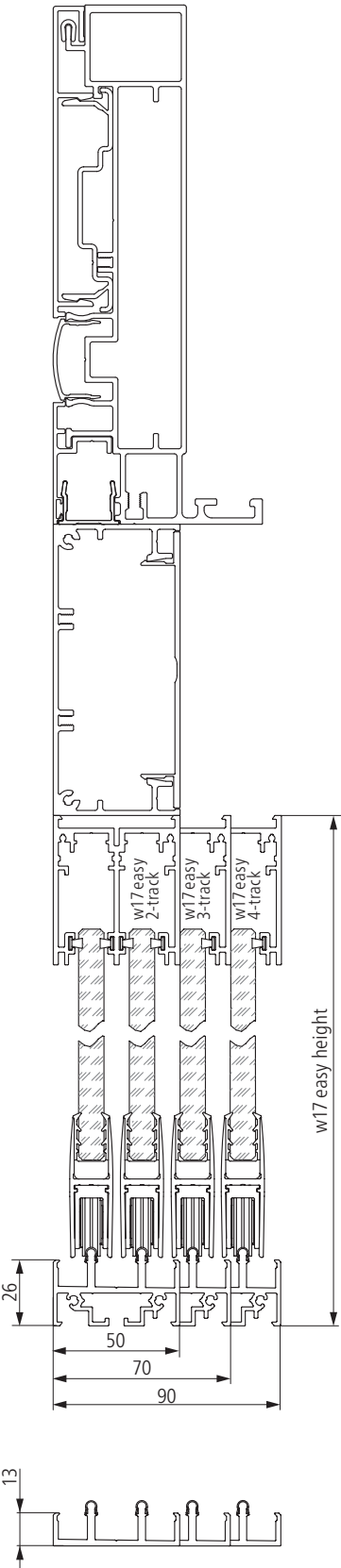
2 to 4-track on one side, 115 x 50 mm frame widener under roof support (retrofitting)
