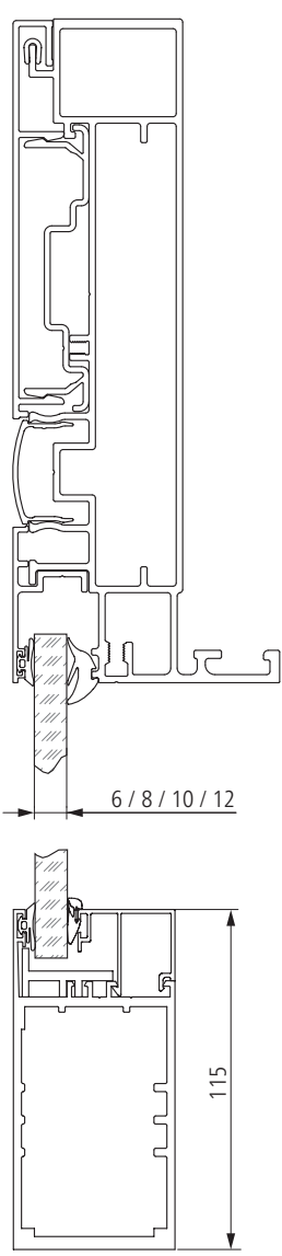
Side roof support with SUPER LITE with 105 mm frame
