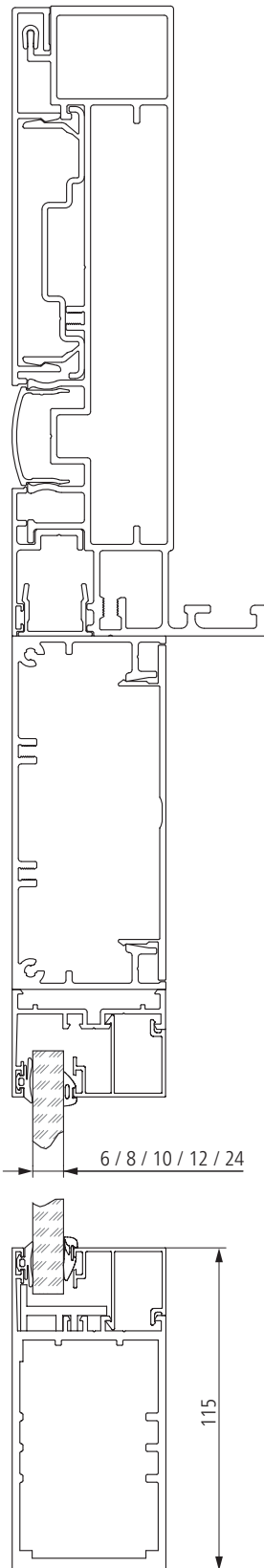
Side roof support with 115 x 50 mm frame widener (for retrofitting) and w50-c SUPER LITE 105 fixed glazing
