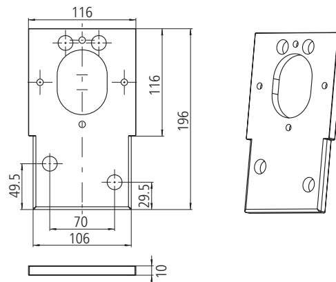
Post plate for 115 middle/wall post
