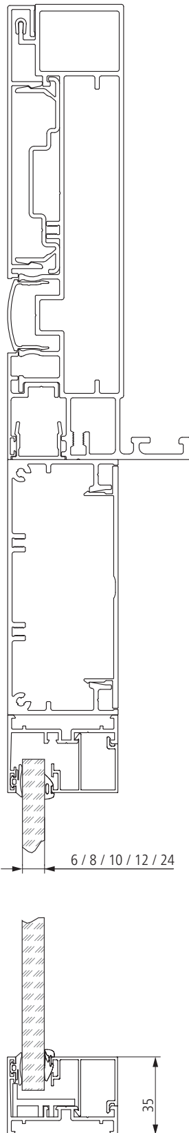
Side roof support with 115 x 50 mm frame widener (for retrofitting) and w50-c SUPER LITE 35 fixed glazing
