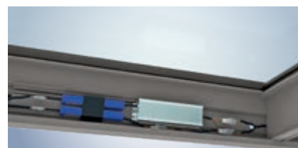
C Wall connection with transformer and pre-assembled plug-in controls for LED color strips
