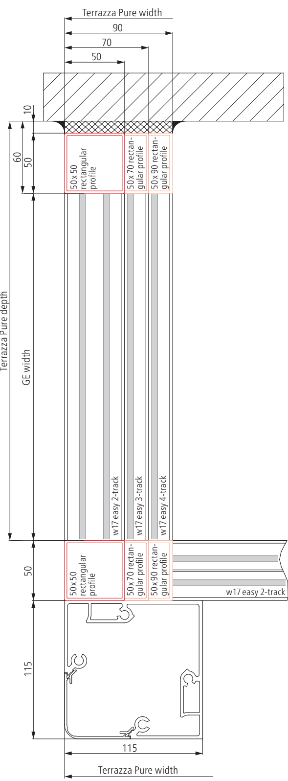
2 to 4-track on one side, 2-track at the front
