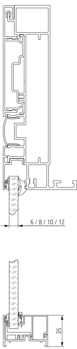
Side roof support with SUPER LITE with 35 mm frame
