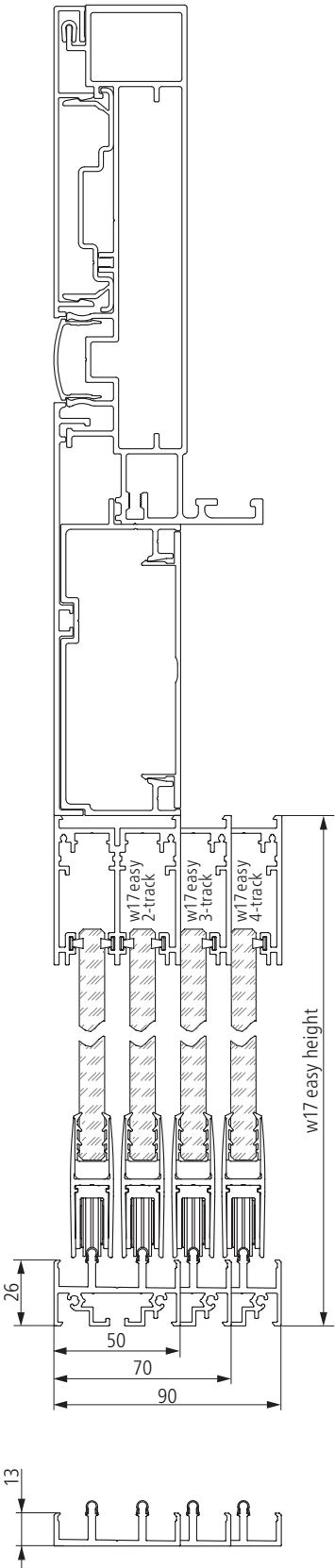
2 to 4-track on one side, 163 x 50 mm frame widener under roof support (standard)
