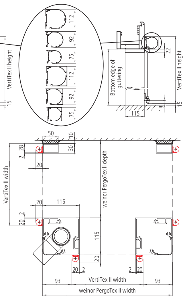
Top view of the VertiTex II rope guide on the weinor PergoTex II (front and side)
