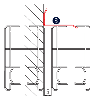
"Small" wall bracket 3 , for unit 2 with drive on the right M (lateral spacing of 5 mm)
