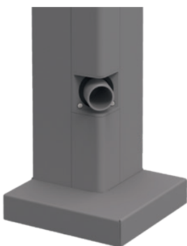
Post base L, external t=15 / t=25 with external post cover cap
