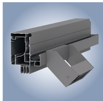
Frame profile short side with Tempura Quadra on guttering when combined with w17 easy
