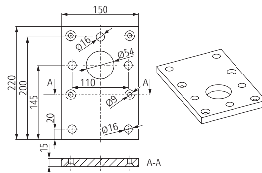
Post plate post 220x150x15
