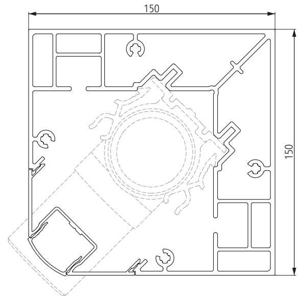
Corner post with decorative strip
