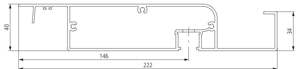
LED louvre
