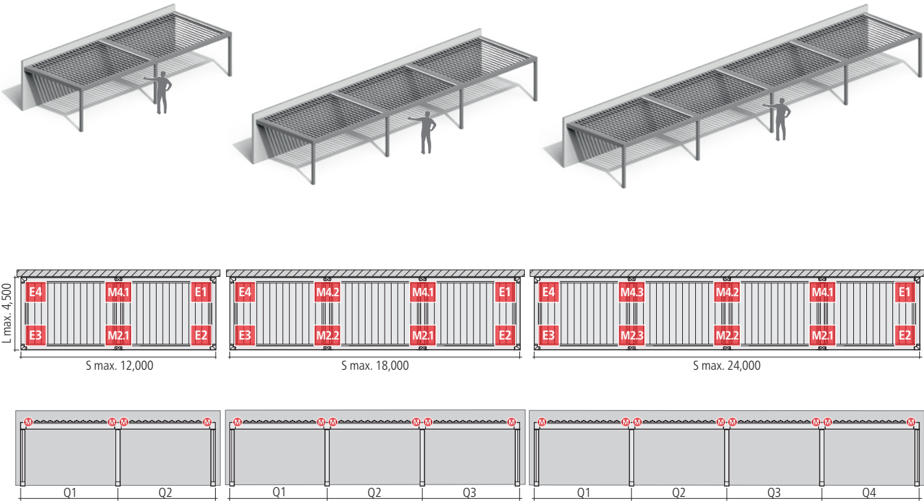
2-section unit
