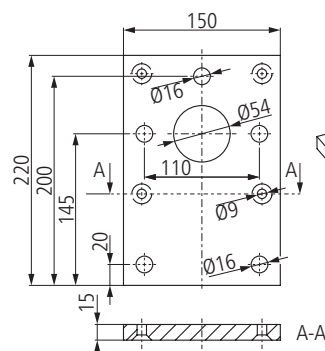
Post plate post 220x150x15
