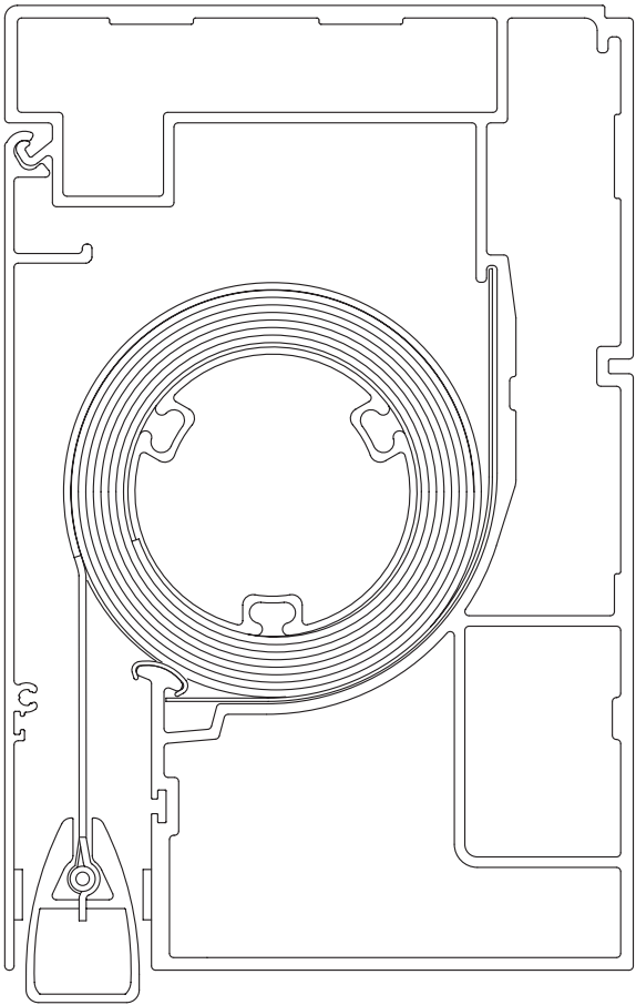
Vertical sun protection retracted
