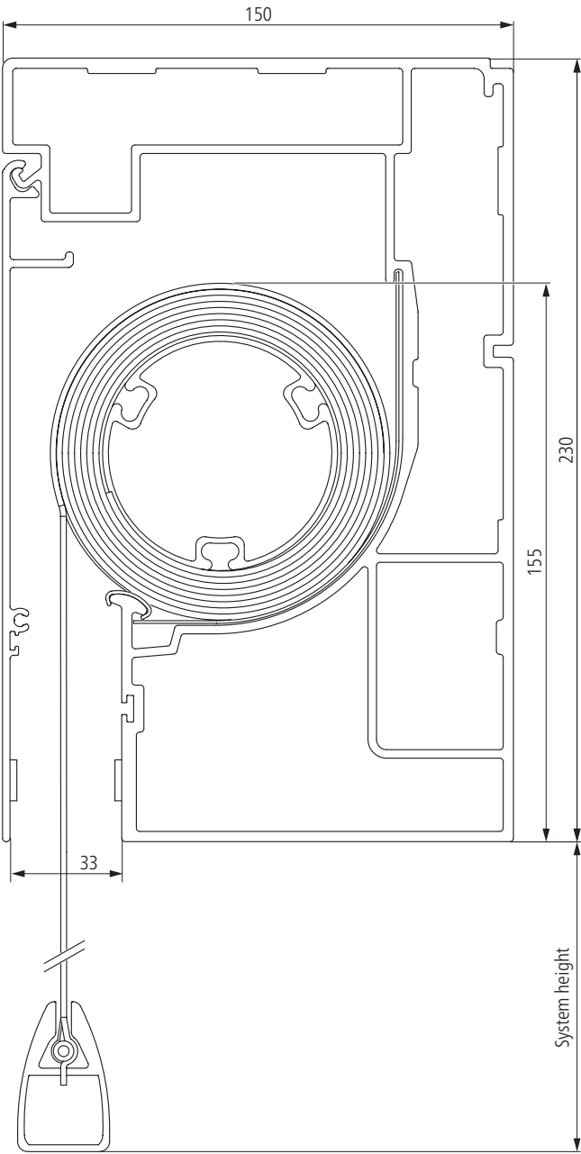
Vertical sun protection extended (frame bottom edge up to OKFF)
