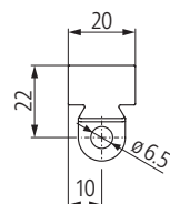
VertiTex 38 x 20 x 32 mm standard rope holder
