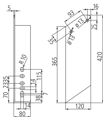
Rafter bracket
