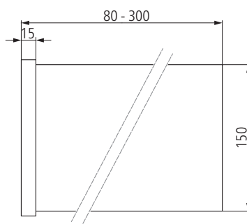
Stand off bracket with wall bracket 180 mm
