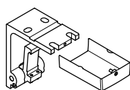
Top fixture bracket incl. decorative cover
