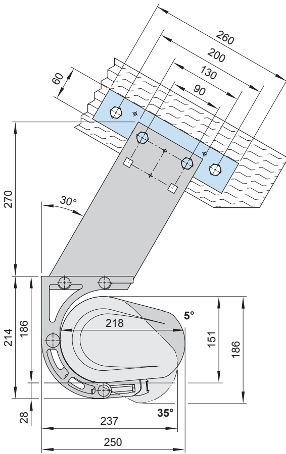
With eaves fixture bracket 270 mm (77940.)
