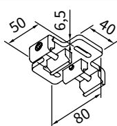
double track bracket flat
