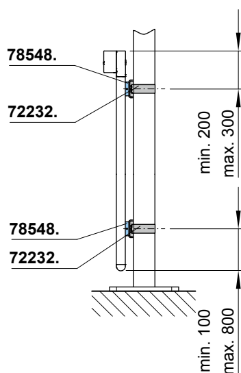
post fixture guide track single and double bracket square post
