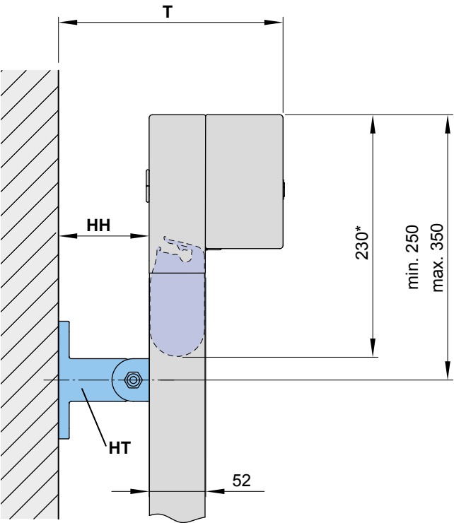
Dimension overview
