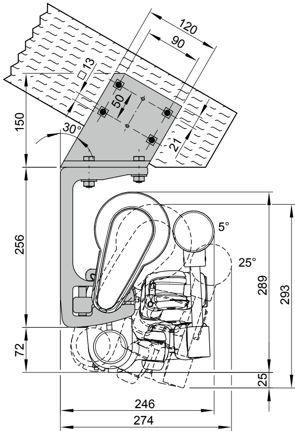
with eaves fixture bracket, 150 mm plate (71612.)
