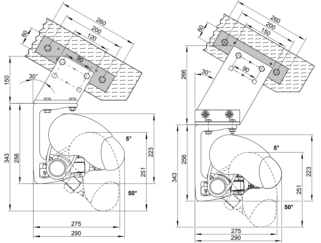
With eaves fixture bracket 150 mm (71612.)
