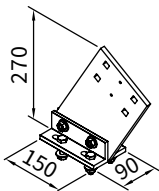
eaves fixture bracket
