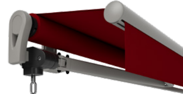
3 pitch adjustment mechanism 1)
